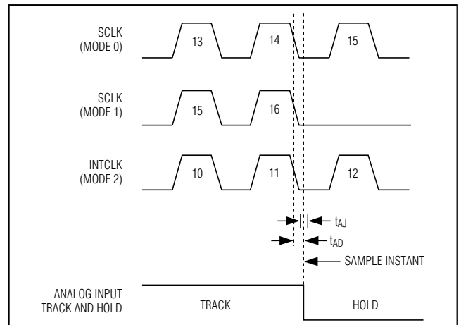
Figure 21. Aperture Diagram
