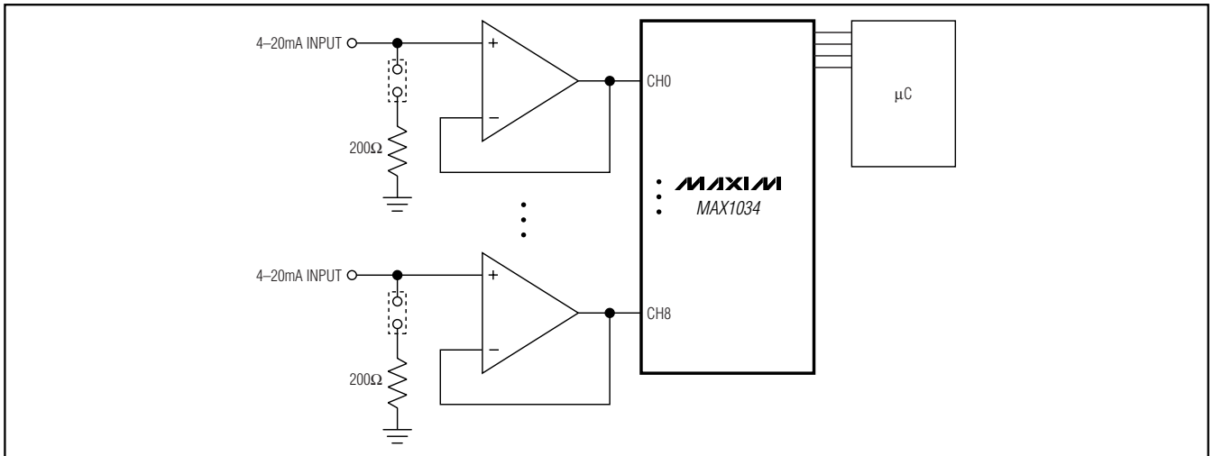
Figure 19. 4-20mA Application
