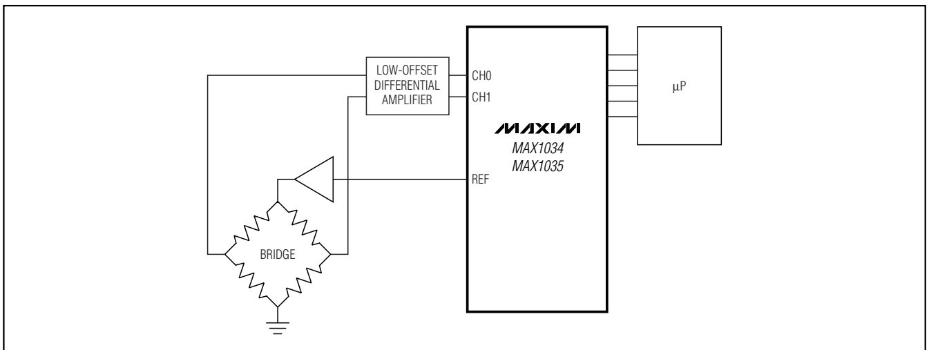
Figure 20. Bridge Application
